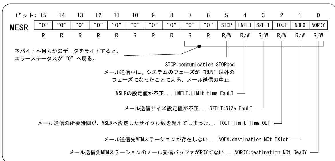
図4.25 MESR
