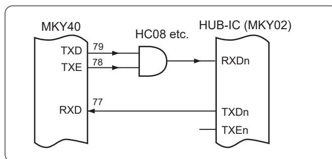
Fig. 3.6 Example of Direct Connection to HUB-IC
