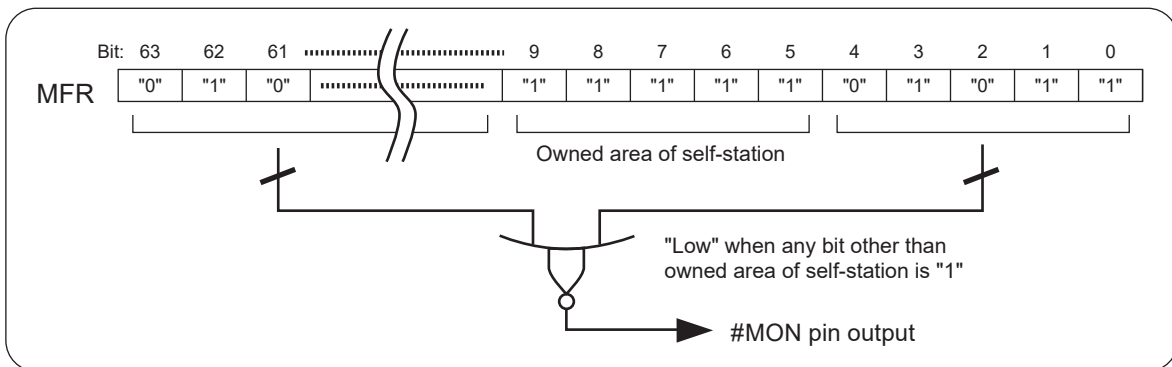
Fig. 4.35 Example of Output to #MON Pin
