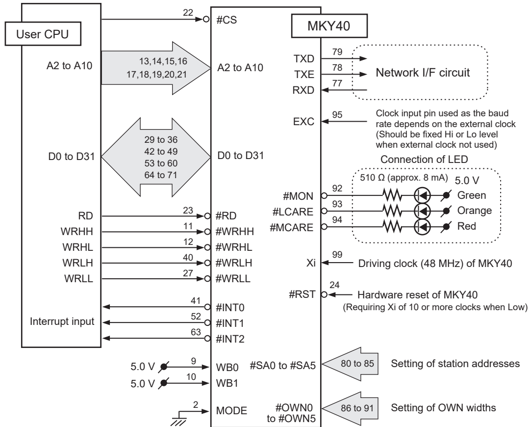
Fig. 3.11 Connection to 32-bit Wide User CPU
