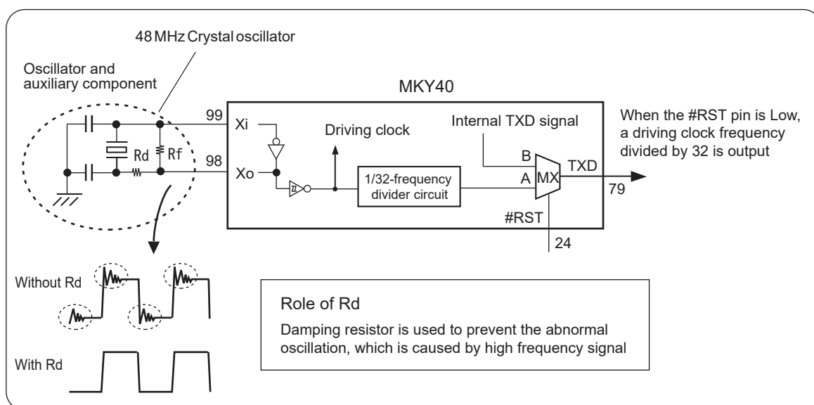
Fig. 3.1 Self-generation of Driving Clock
