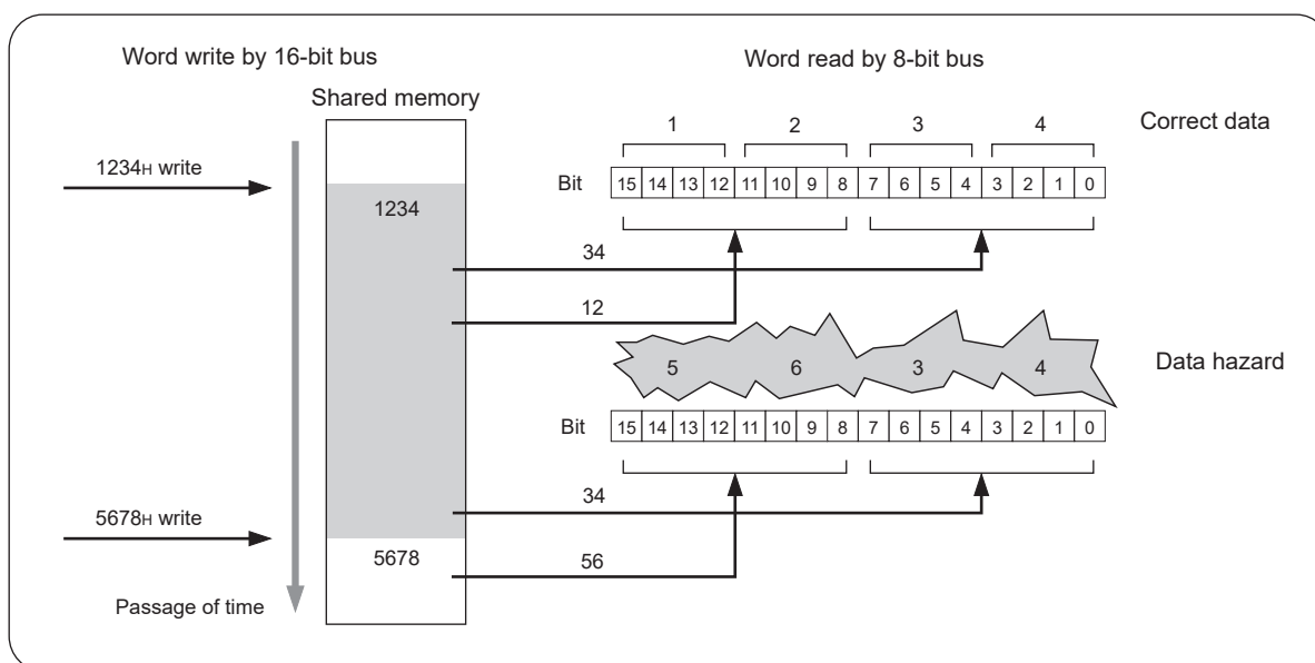
Fig. 4.7 Mechanism of Data Hazard
