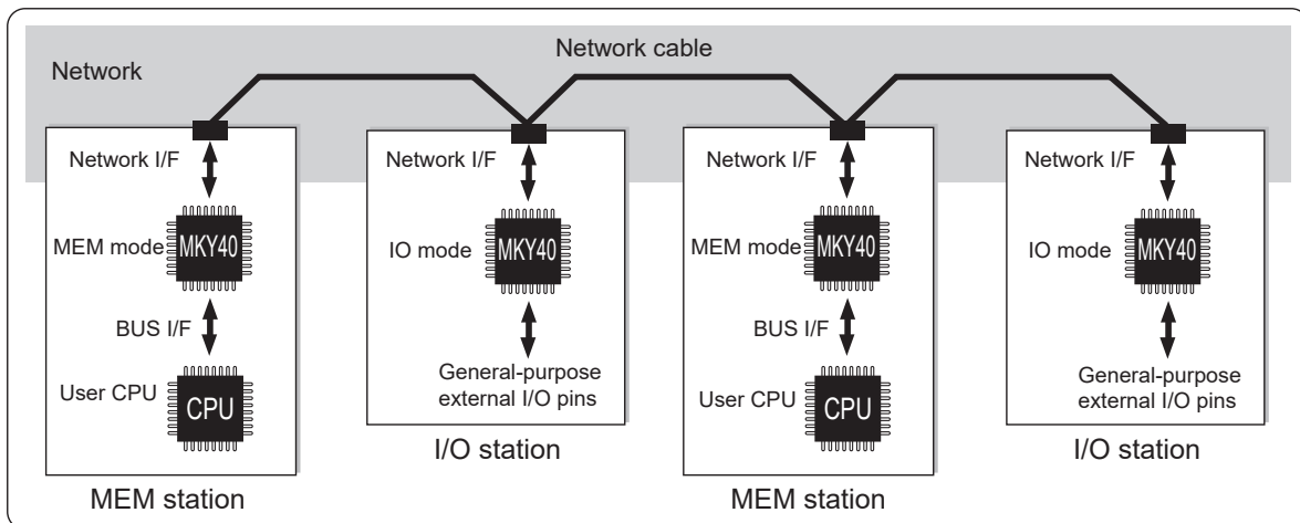
Fig. 1.4 CUnet Connecting Two Modes
