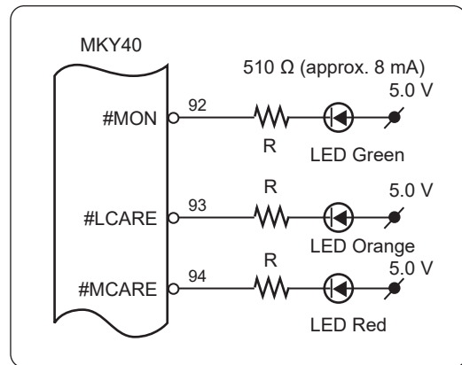
Fig. 3.10 Example of LED Display Pin Connection
