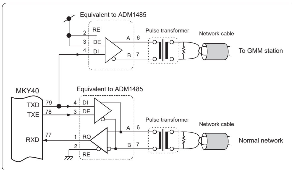
Fig. 3.5 Example of Adding Cable for GMM Station
