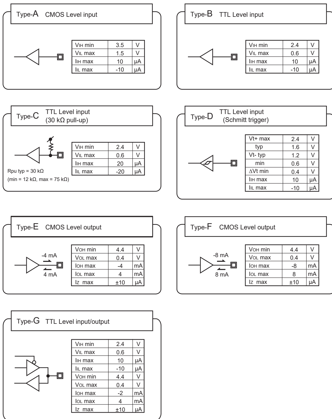
Fig. 6.2 Pin Electrical Characteristics in I/O Circuit Types in IO Mode
