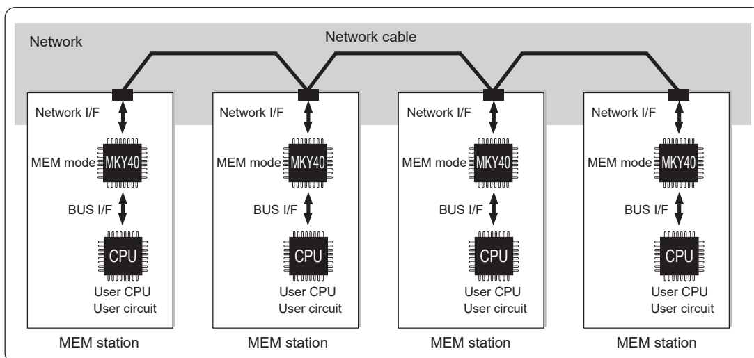
Fig. 1.2 CUNet Connecting Four MEM Stations
