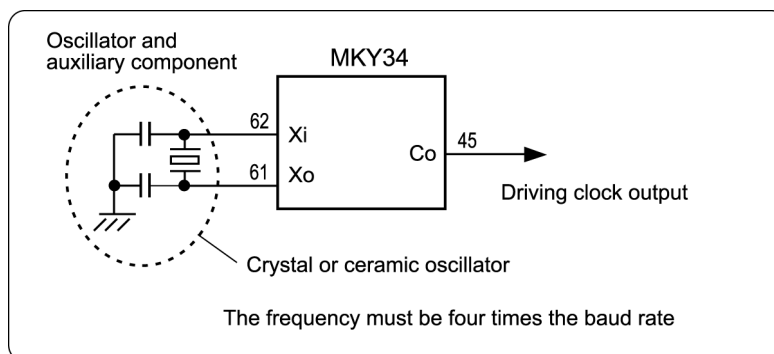
Fig. 3.1 Connecting Oscillator
