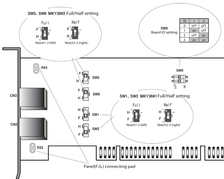
Fig.1-3 Settings of HLSB-36PCI2 board
