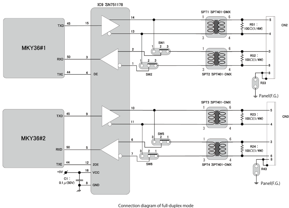
Fig.1-2 Connector peripheral circuit
